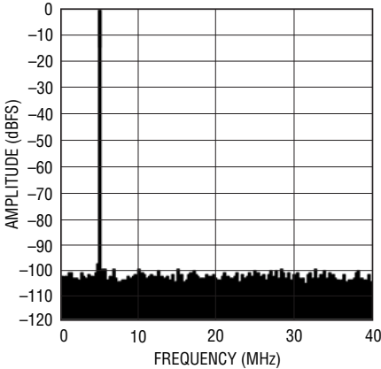
LTC2173-14: 8k Point FFT, f_{IN} = 5\text{MHz} -1\text{dBFS} , 80Msps
