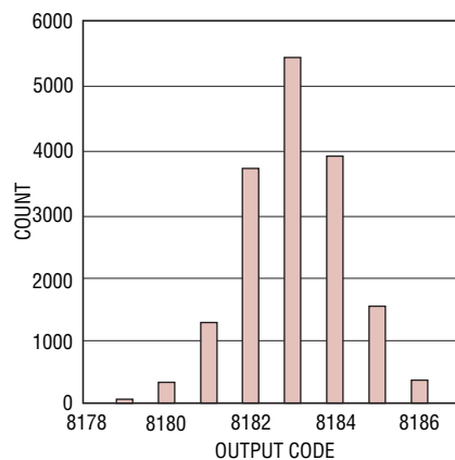
LTC2175-14: Shorted Input Histogram
