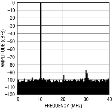
LTC2173-14: 8k Point FFT, f_{IN} = 70\text{MHz} -1\text{dBFS} , 80Msps
