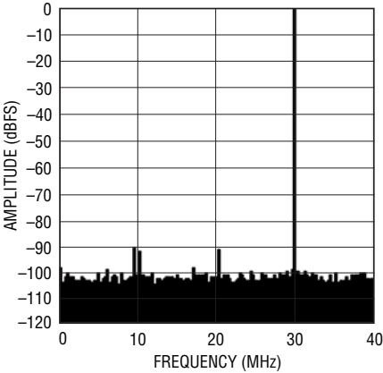
LTC2173-14: 8k Point FFT, f_{IN} = 30\text{MHz} -1\text{dBFS} , 80Msps
