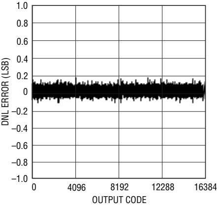
LTC2173-14: Differential Nonlinearity (DNL)
