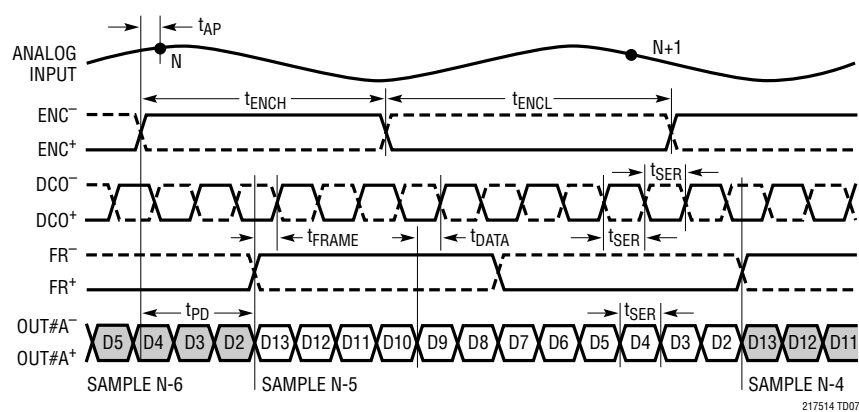
One-Lane Output Mode, 12-Bit Serialization
