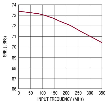
LTC2175-14: SNR vs Input Frequency, -1dB, 2V Range, 125Msps
