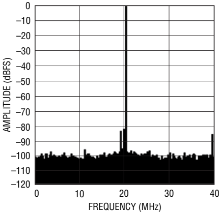
LTC2173-14: 8k Point FFT, f_{IN} = 140\text{MHz} -1\text{dBFS} , 80Msps
