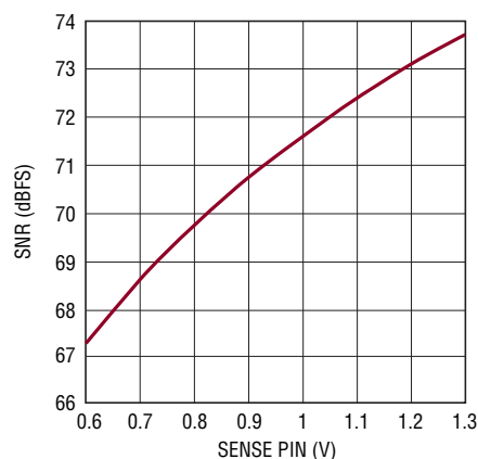
LTC2175-14: SNR vs SENSE, f_{IN} = 5\text{MHz} , -1dB
