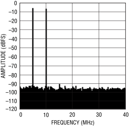
LTC2173-14: 8k Point 2-Tone FFT, f_{IN} = 70\text{MHz} , 75MHz, -1\text{dBFS} , 80Msps
