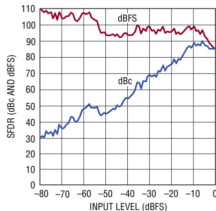
LTC2174-14: SFDR vs Input Level, f_{IN} = 70\text{MHz} , 2V Range, 105Mpsps
