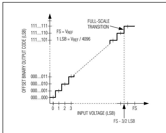
Figure 3. Unipolar Transfer Function—Full Scale (FS) = V_{\text{REF}}
