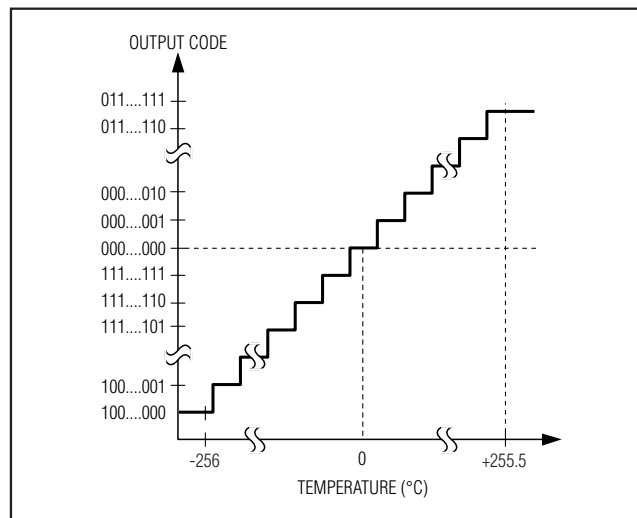
Figure 5. Temperature Transfer Function
