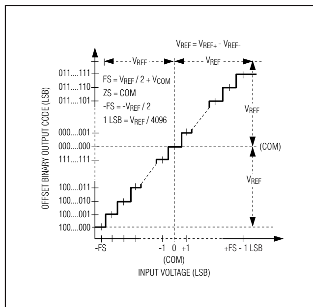
Figure 4. Bipolar Transfer Function—Full Scale ( \pm\text{FS} ) = \pm V_{\text{REF}} / 2
