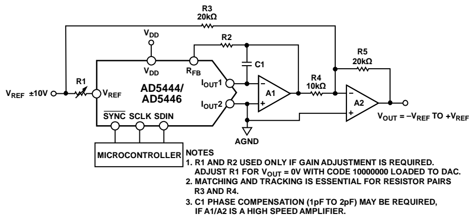
Figure 39. Bipolar Operation (4-Quadrant Multiplication)
