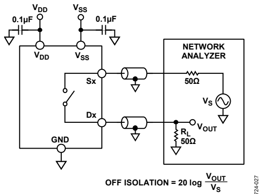
Figure 34. Off Isolation
