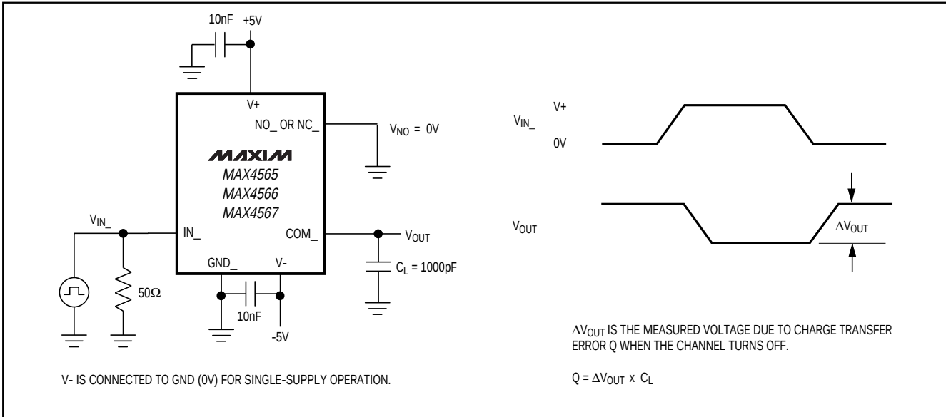
Figure 5. Charge Injection
