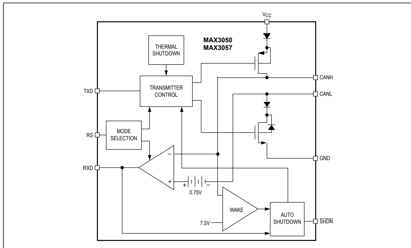
Figure 4. Functional Diagram
