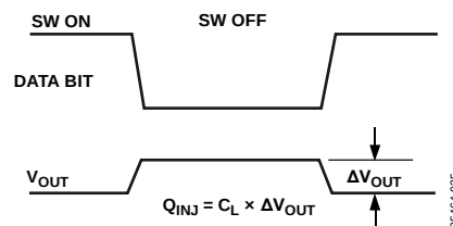
Figure 29. Charge Injection
