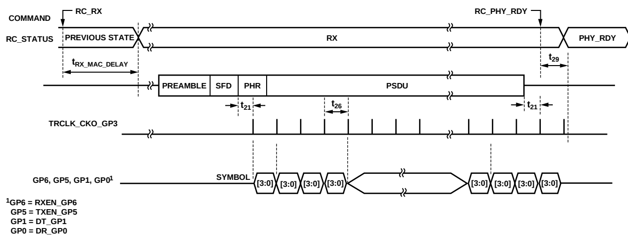
Figure 8. IEEE 802.15.4 RX SPORT Mode: Symbol Clock Output
