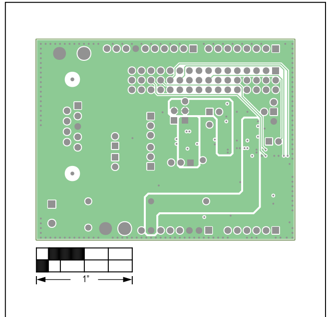
MAX13053A Shield—Internal 3
