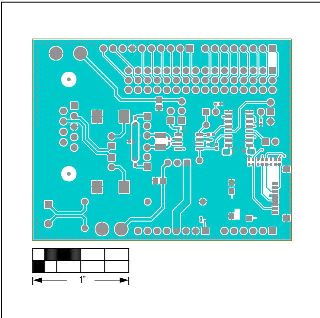
MAX13053A Shield—Top
