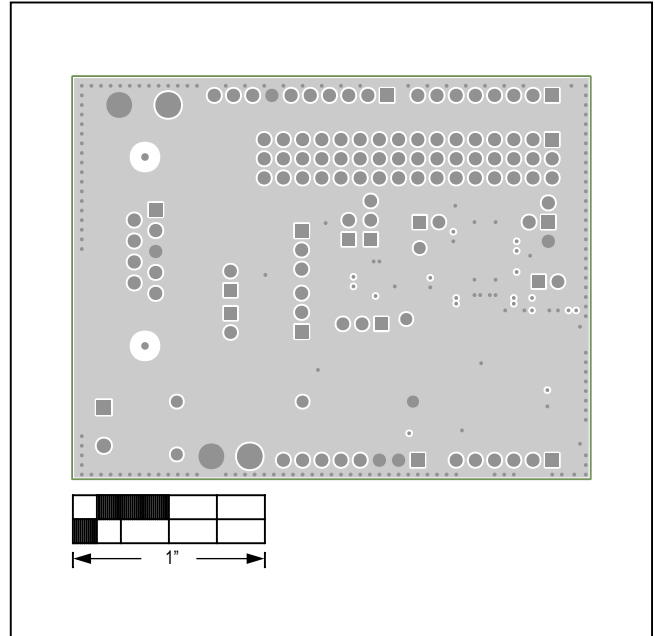
MAX13053A Shield—Internal 2
