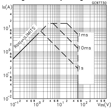
Figure 2: Safe operating area
