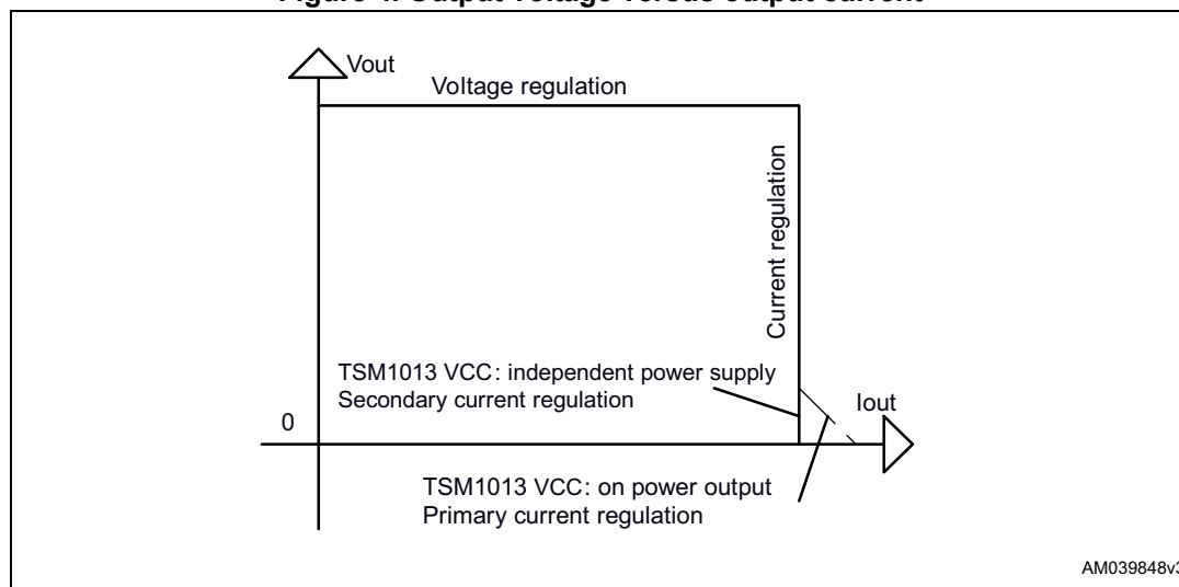
Figure 4. Output voltage versus output current
