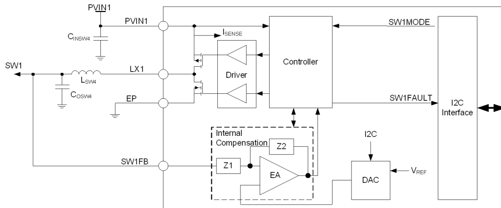
Figure 9. SW1 diagram
