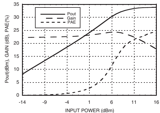
Power Compression @ 8 GHz, 7V @ 1340 mA
