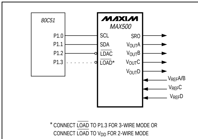
Figure 13. 80C51 Interface
