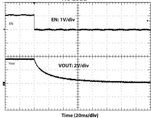
Vout Disabled Operation: SC33001A, V_{in}=3.6V No Load
