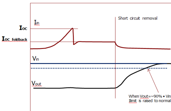
Figure 1 — Startup into Short Circuit and Recovery from Short Circuit Removal Behavior
