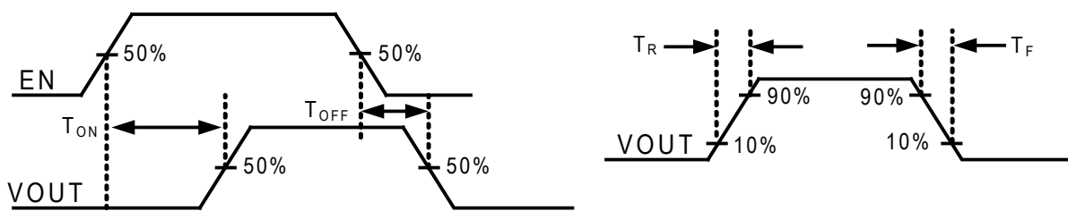
T_{ON} , T_{OFF} , T_R , T_F WAVEFORMS
