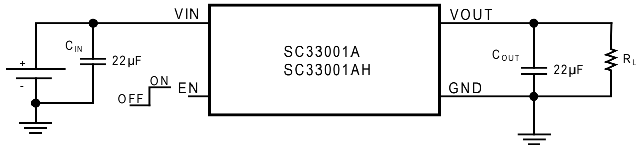
TEST CIRCUIT
