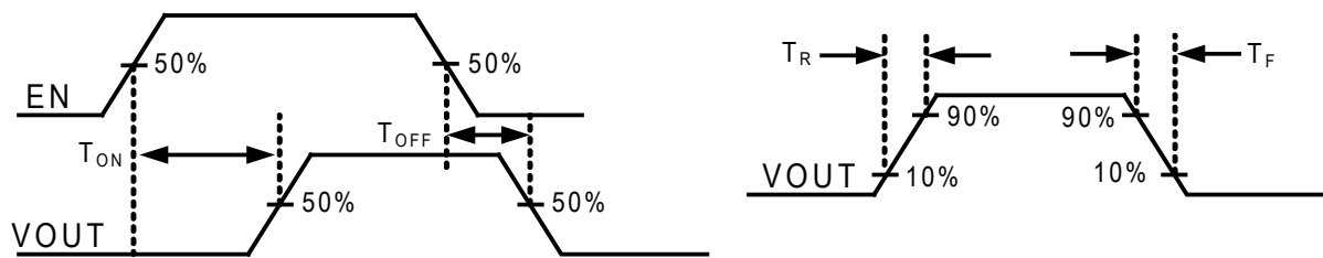
T_{\text{ON}} , T_{\text{OFF}} , T_R , T_F WAVEFORMS
