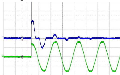
Figure 5- Inrush current, V_{in} = 230V_{ac} , 90^\circ CH4: V_{in} (200V/div), CH3: I_{in} (20A/div)
