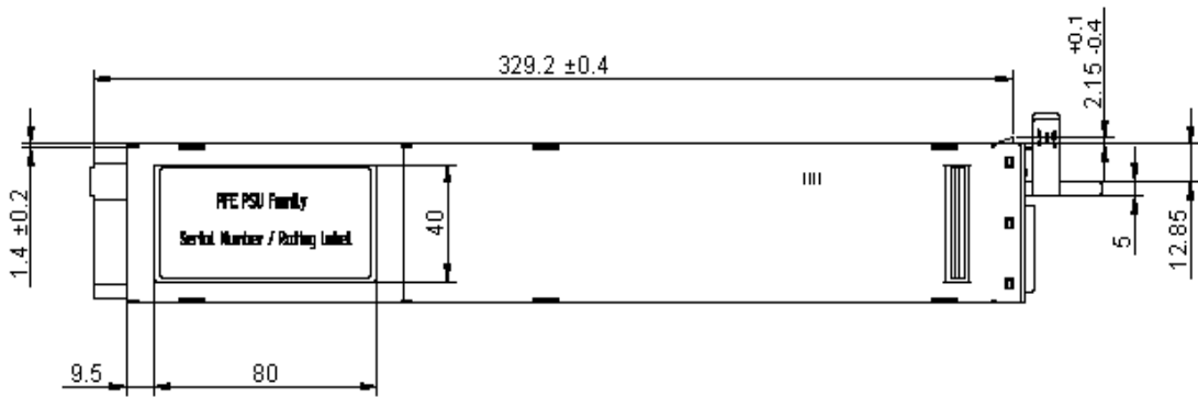
Figure 44 - Top View
