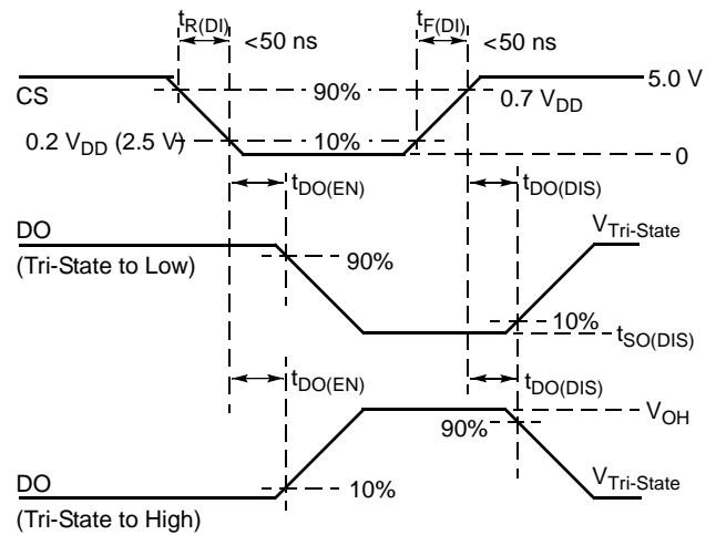
Figure 11. Turn-ON/OFF Waveforms
