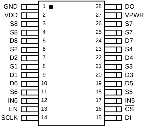
Figure 3. 28-Pin Connections
