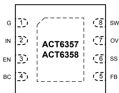
TDFN33-8
