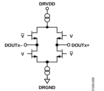
Figure 29. Equivalent Digital Output Circuit
