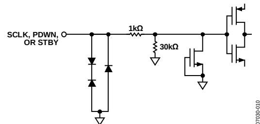
Figure 30. Equivalent SCLK, PDWN, or STBY Input Circuit
