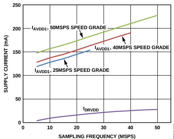
Figure 61. Supply Current vs. f_{\text{SAMPLE}} for f_{\text{IN}} = 5 \text{ MHz}
