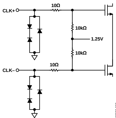
Figure 27. Equivalent Clock Input Circuit
