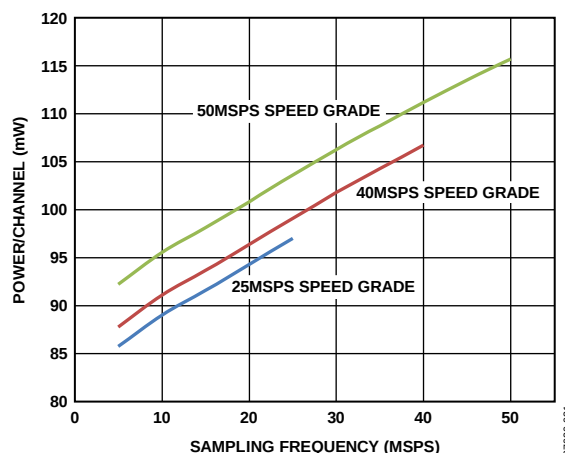
Figure 62. Power per Channel vs. f_{\text{SAMPLE}} for f_{\text{IN}} = 5 \text{ MHz}
