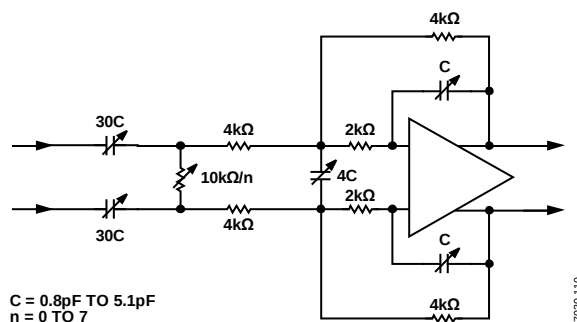
Figure 54. Simplified Filter Schematic
