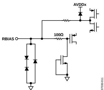
Figure 31. Equivalent RBIAS Circuit
