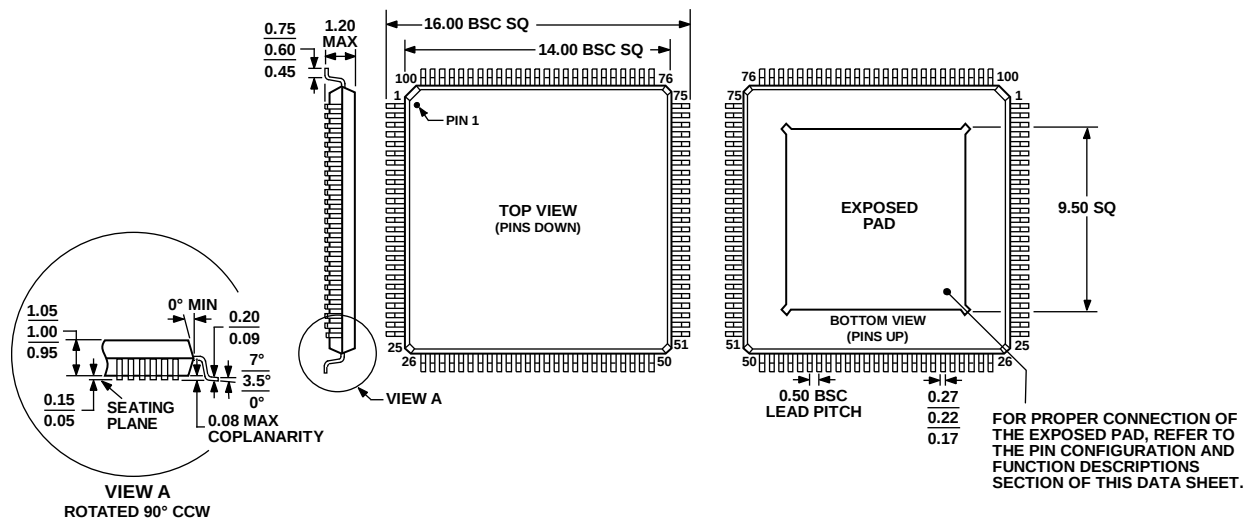
Figure 71. 100-Lead Thin Quad Flat Package, Exposed Pad [TQFP_EP] (SV-100-3)
