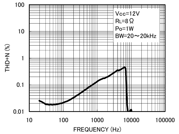
Fig. 2 THD+N – Frequency
