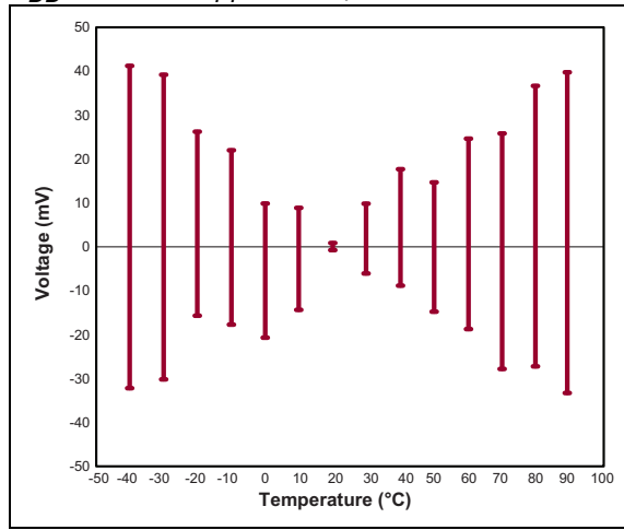
FIGURE 2-4: Distribution of Typical HV_{OUT} Deviation over Temperature ( V_{IN} = 0.1 V_{DC} , 1.6 V_{DC} , 3.3 V_{DC} , in reference to 20°C).
