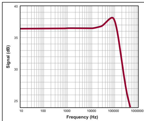
FIGURE 2-3: Typical Bode Plot of Small-signal Gain ( V_{IN} = 0.2 V_{P-P} , V_{DC} = 1.5V , V_{DD} = 5V and V_{PP} = 200V ).
