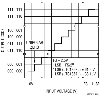
Figure 9. LTC1863L/LTC1867L Unipolar Transfer Characteristics (Straight Binary)
