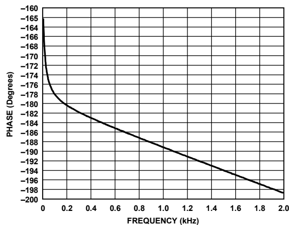
Figure 45. Phase vs. Frequency, 2 kHz Bandwidth f_s = 786 kHz, Signal Path = DAC_SDATx to ASRC to LOU TLx
