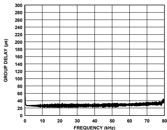
Figure 44. Group Delay vs. Frequency, f_s = 786 kHz, Signal Path = DAC_SDATx to ASRC to LOU TLx
