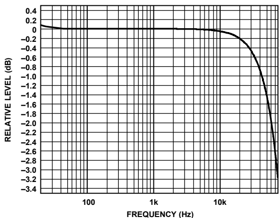
Figure 41. Relative Level vs. Frequency, f_s = 786 kHz, Signal Path = DAC_SDATx to ASRC to LOU TLx
