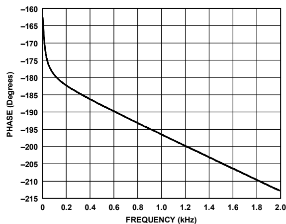
Figure 43. Phase vs. Frequency, 2 kHz Bandwidth, f_s = 192 kHz, Signal Path = DAC_SDATx to ASRC to LOU TLx
