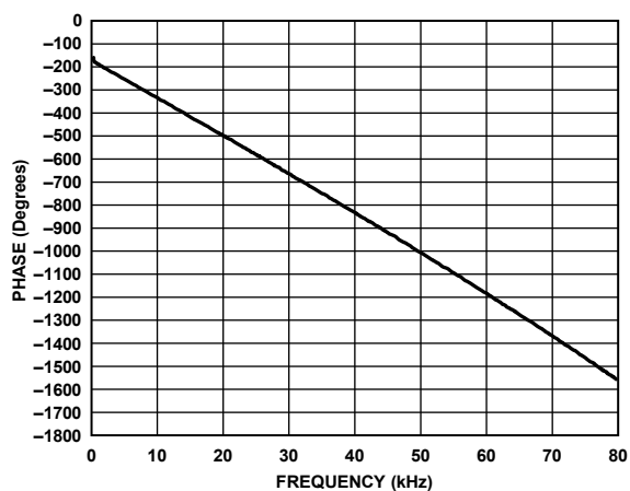
Figure 40. Phase vs. Frequency, 80 kHz Bandwidth, f_s = 192 kHz, Signal Path = DAC_SDATx to ASRC to LOU TLx
