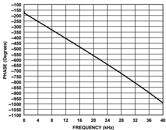
Figure 42. Phase vs. Frequency, 20 kHz Bandwidth, f_s = 786 kHz, Signal Path = DAC_SDATx to ASRC to LOU TLx
