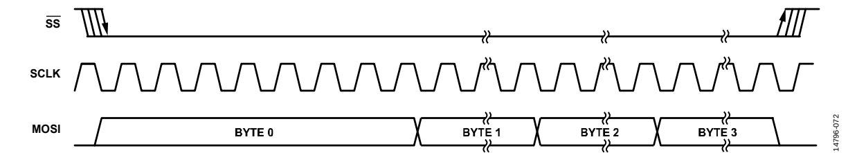
Figure 64. SPI Write to ADAU1777 Clocking (Single Write Mode)
