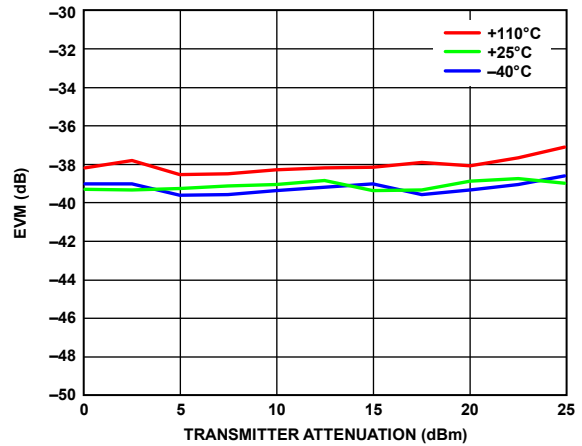
Figure 373. EVM vs. Transmitter Attenuation, LTE Signal = 20 MHz, Centered on DC, LO = 5900 MHz
