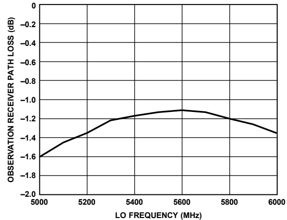
Figure 374. Observation Receiver Path Loss vs. LO Frequency, Can be Used for De-Embedding Performance Data
