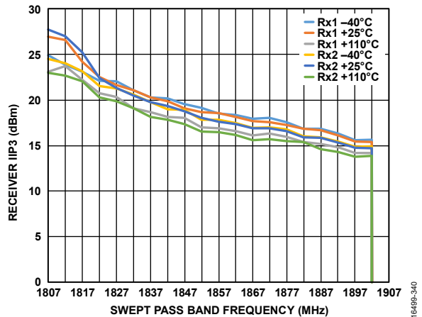
Figure 217. Receiver IIP3 vs. Swept Pass Band Frequency, Receiver Attenuation = 0 dB, LO = 1800 MHz, Tone 1 = 1802 MHz, Tone 2 = Swept Across Pass Band, -21 dBm Each
