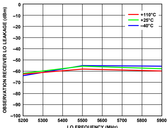
Figure 375. Observation Receiver LO Leakage vs. LO Frequency LO = 5200 MHz, 5500 MHz, and 5900 MHz
