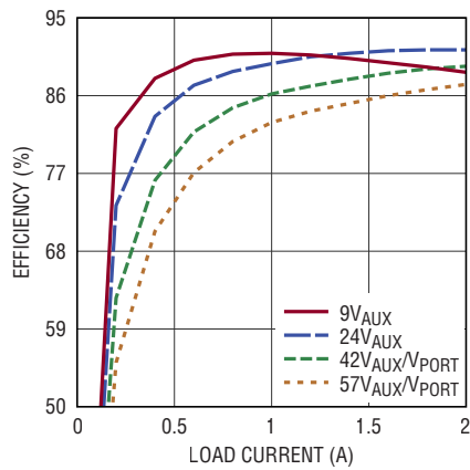
Figure 2. Efficiency (End-to-End)
