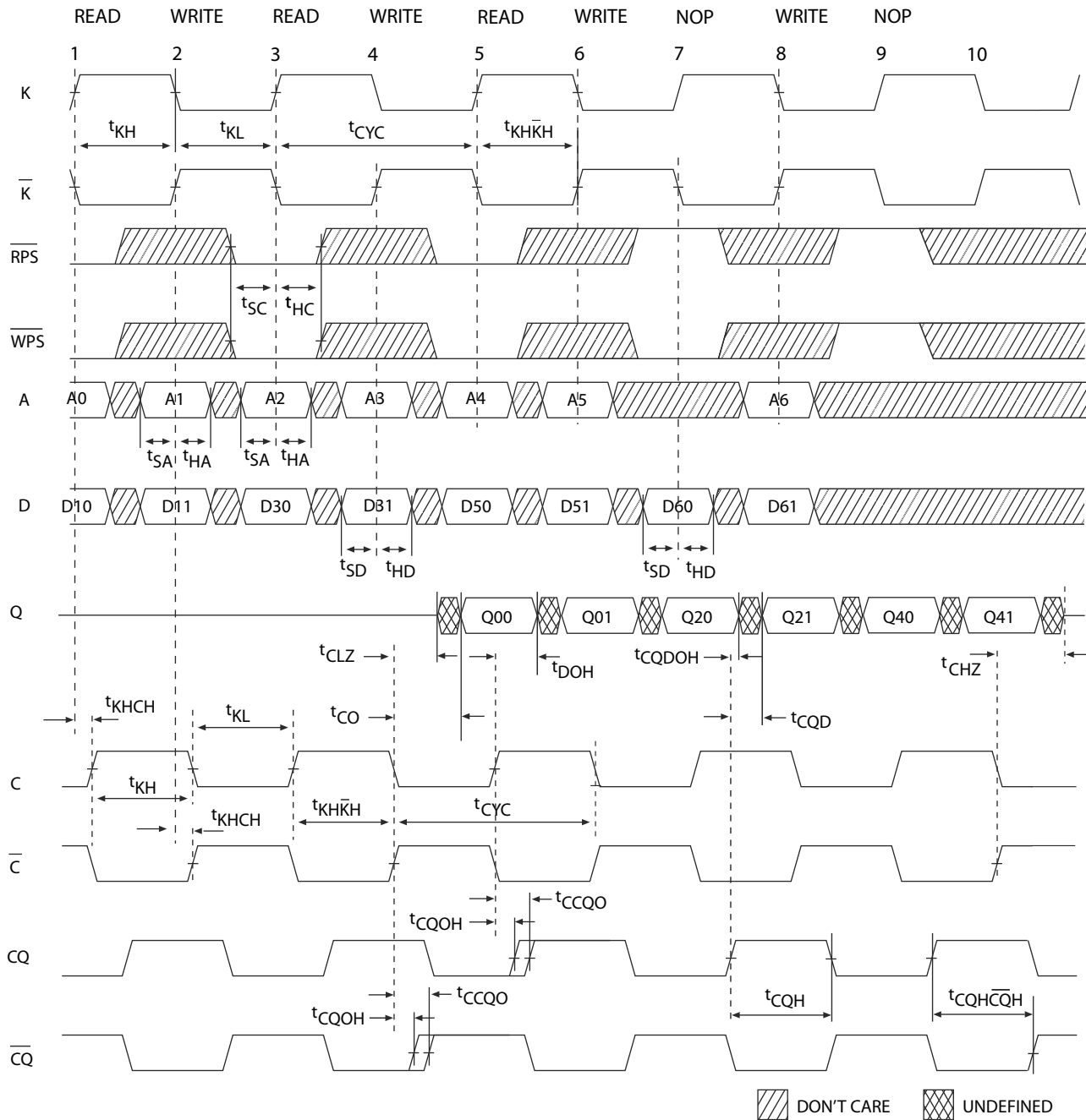
Figure 6. Read/Write/Deselect Sequence [36, 37, 38]
