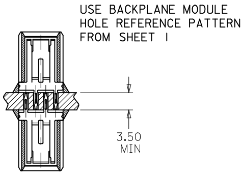
BACK-TO-BACK MOUNTING APPLICATION
