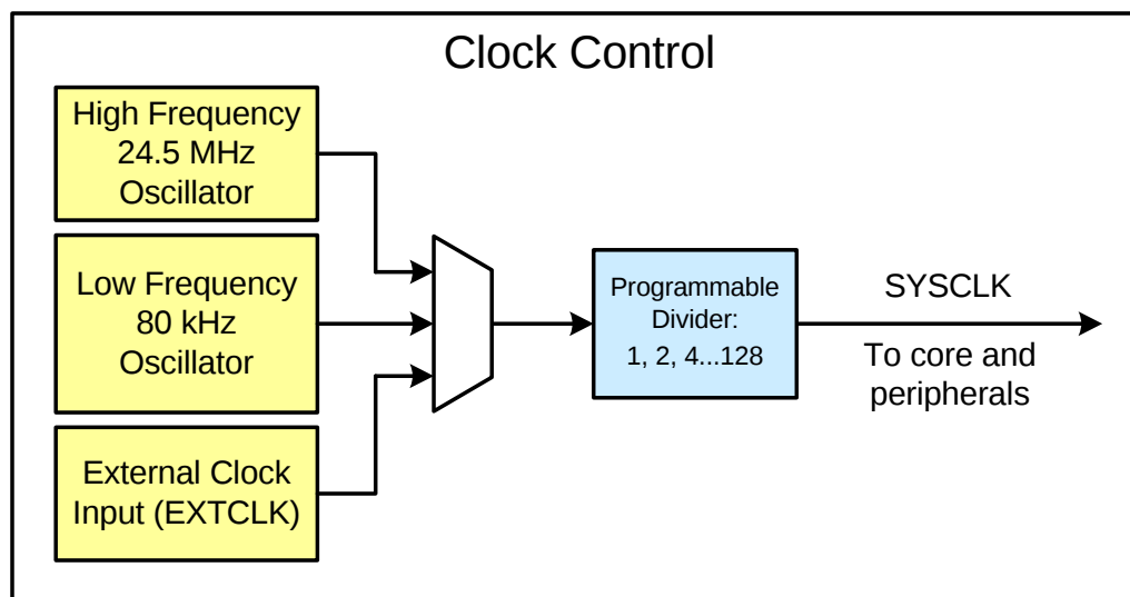
Figure 16.1. Clocking Options
