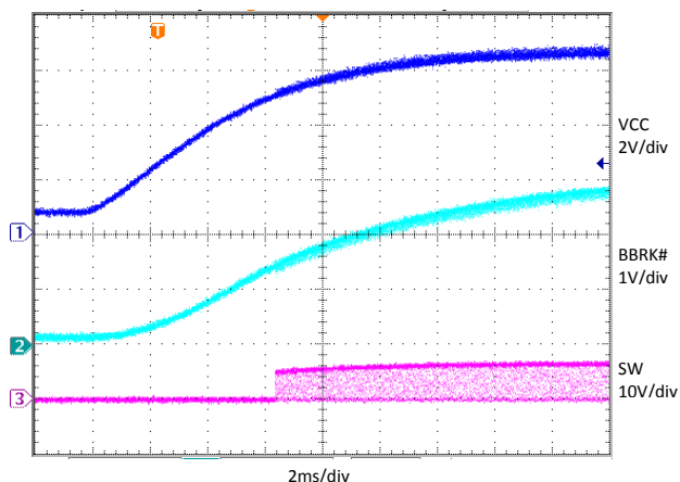
Figure 24: Diode Emulation Setup through BBRK# Capacitor
