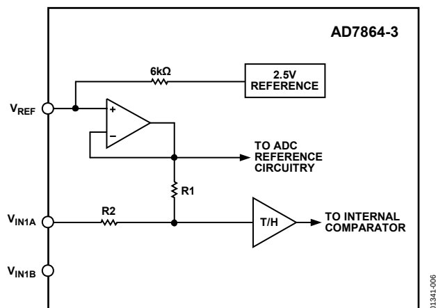
Figure 6. AD7864-3 Analog Input Structure
