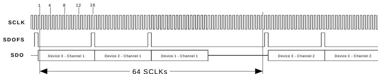
Figure 2. Cascade Timing for a Three-Device Cascade
