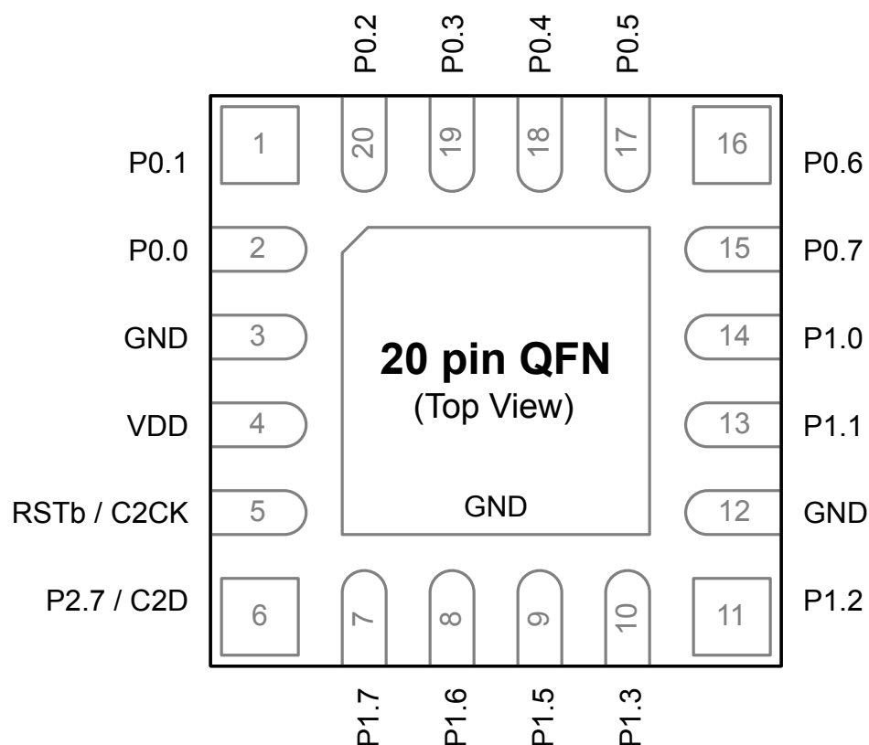
Figure 6.1. EFM8SB1x-QFN20 Pinout
