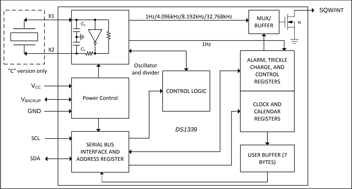
Figure 3. Block Diagram
