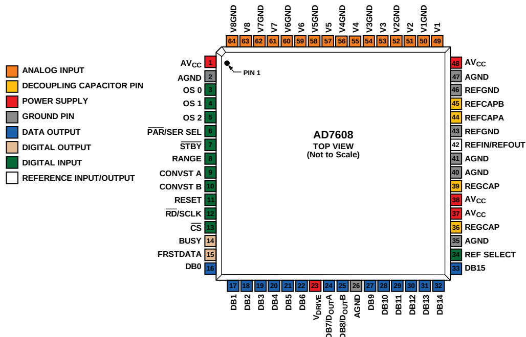
Figure 7. Pin Configuration
