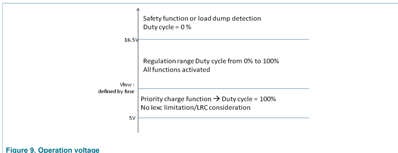
Figure 9. Operation voltage
