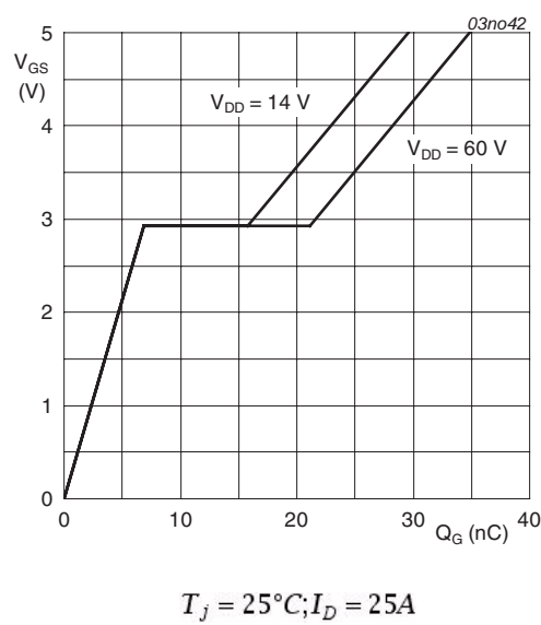
Fig 12. Gate-source voltage as a function of turn-on gate charge; typical values
