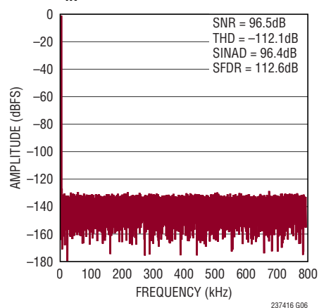
32k Point FFT f_{SAMPL} = 1.6\text{Mpsps} , f_{IN} = 1\text{kHz} , REFBUF = 5\text{V}
