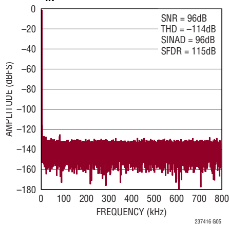
32k Point FFT f_{SAMPL} = 1.6\text{Mpsps} , f_{IN} = 1\text{kHz}
