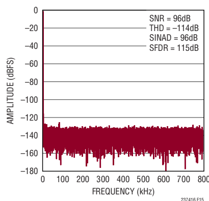
Figure 15. 32k Point FFT f_{\text{SAMPL}} = 1.6\text{Msps} , f_{\text{IN}} = 1\text{kHz}
