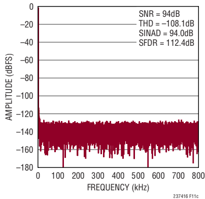
Figure 11c. 32k Point FFT f_{\text{SMPL}} = 1.6\text{Msps} , f_{\text{IN}} = 1\text{kHz} for Circuit Shown in Figure 11b
