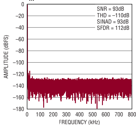
32k Point FFT f_{SAMPL} = 1.6\text{MSPS} , f_{IN} = 1\text{kHz}
