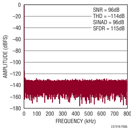
Figure 8b. 32k Point FFT f_{\text{SMPL}} = 1.6\text{Msps} , f_{\text{IN}} = 1\text{kHz} for Circuit Shown in Figure 8a; Driven with Fully Differential Inputs
