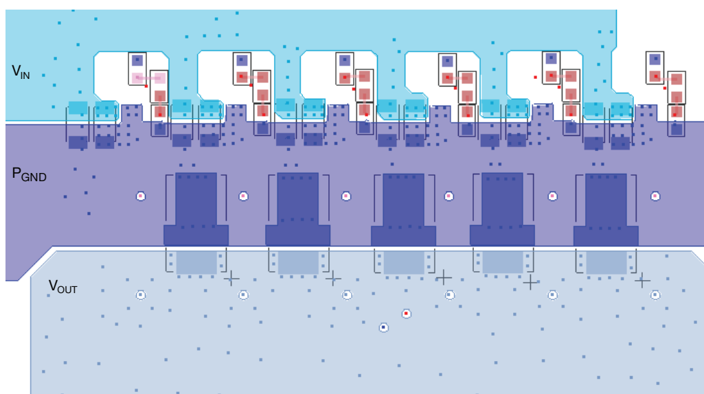
Fig. 19 - Multi - Phase VRPower Layout Bottom View
