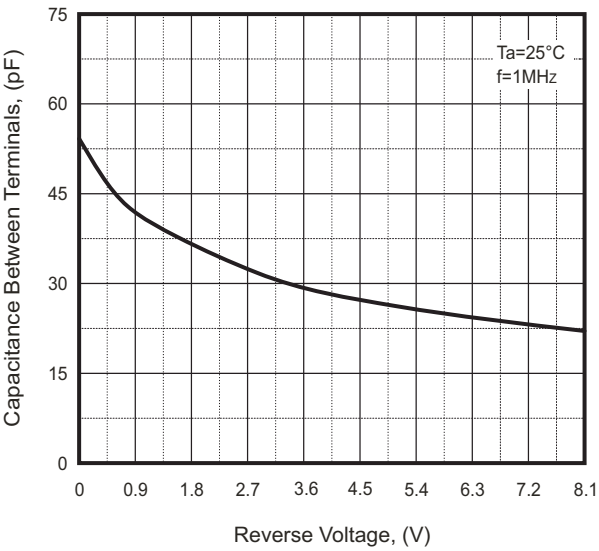
Fig.4 - Capacitance Characteristics
