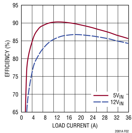
Figure 2. Measured LTM4630-1 Efficiency ( V_{OUT} = 1.0V , f_{sw} = 400kHz )
