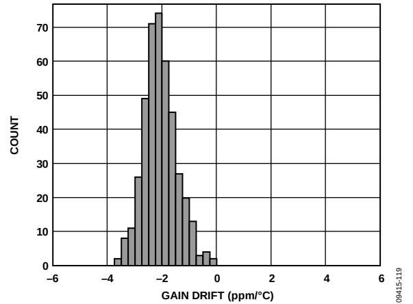
Figure 24. Gain Drift Distribution
