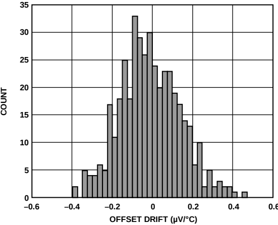
Figure 25. Input Offset Drift Distribution
