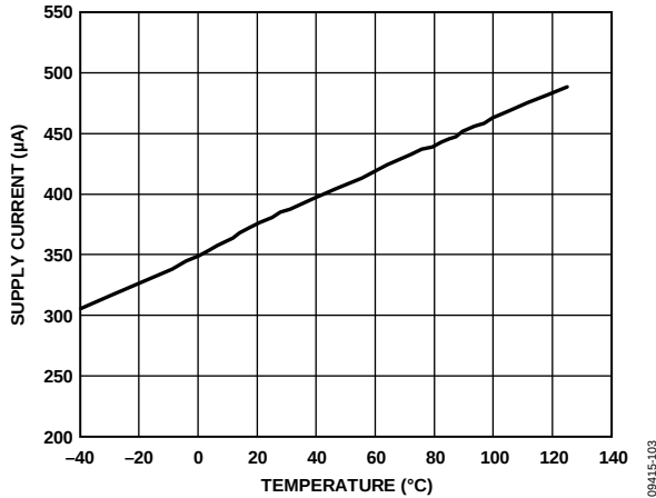
Figure 10. Typical Supply Current Change over Temperature ( V_S = 5V )
