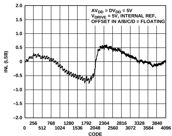
Figure 20. DAC INL
